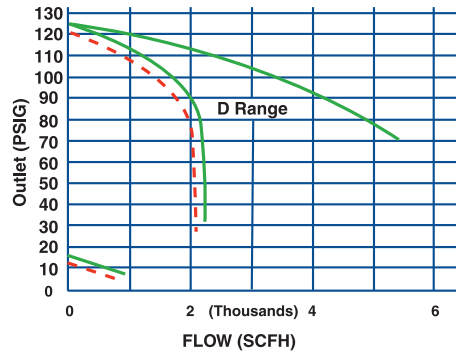
FLOW DATA (Flowing Air at STD. Conditions)
